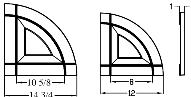
14 3/4 x 14 3/4 Raised Panel
